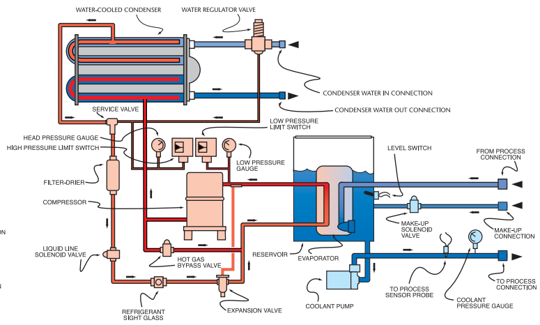
Schematic is typical of 5 to 40 ton models. See standard features list for details. Hot gas bypass valve is excluded on units with Digital Scroll compressor.
